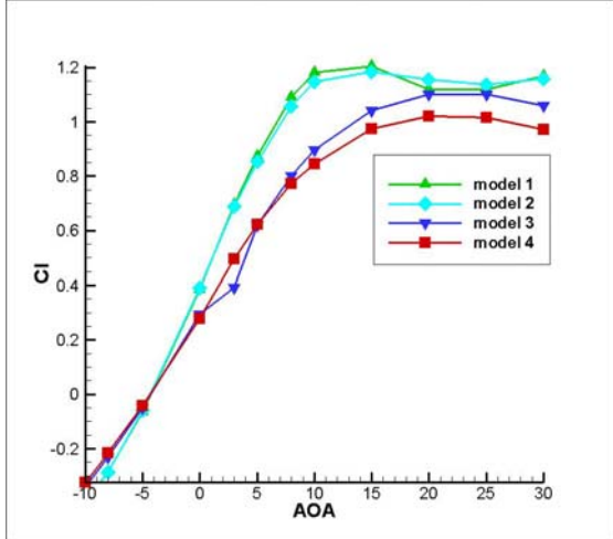
Fig. 9: Lift coefficients vary with AOA changes
