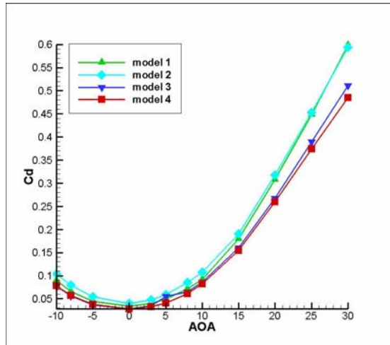
Fig. 8: Drag coefficients vary with AOA changes
