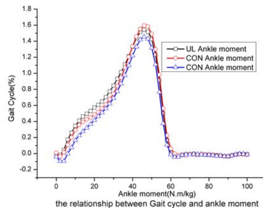
Fig.7: Ankle Moment
