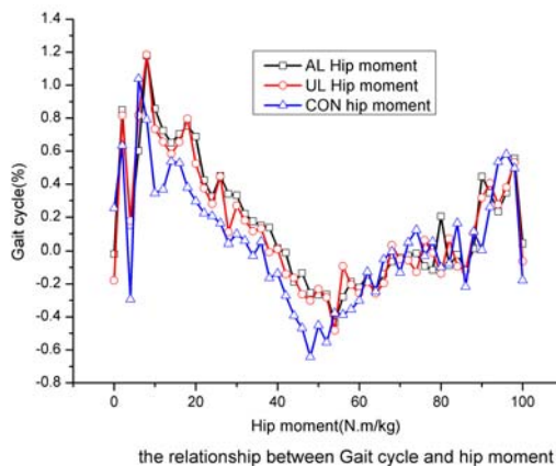
Fig.6: Hip Moment
