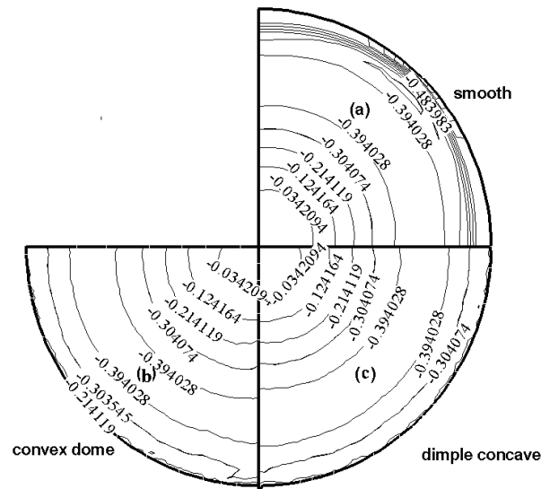
Fig. 8: The static pressure isoline of the model
