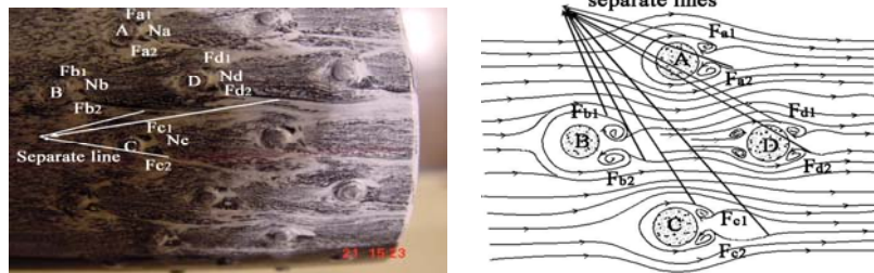
Fig. 5: Oil pattern at the wind speed is 38m/s and attack angle is 0^\circ
