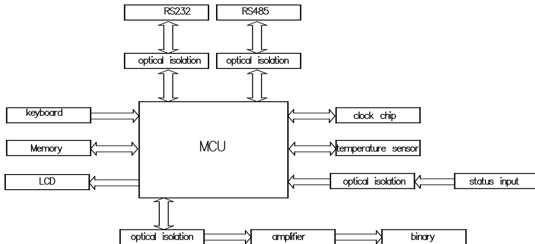
Figure 3: The structure of the single chip microcomputer system software
