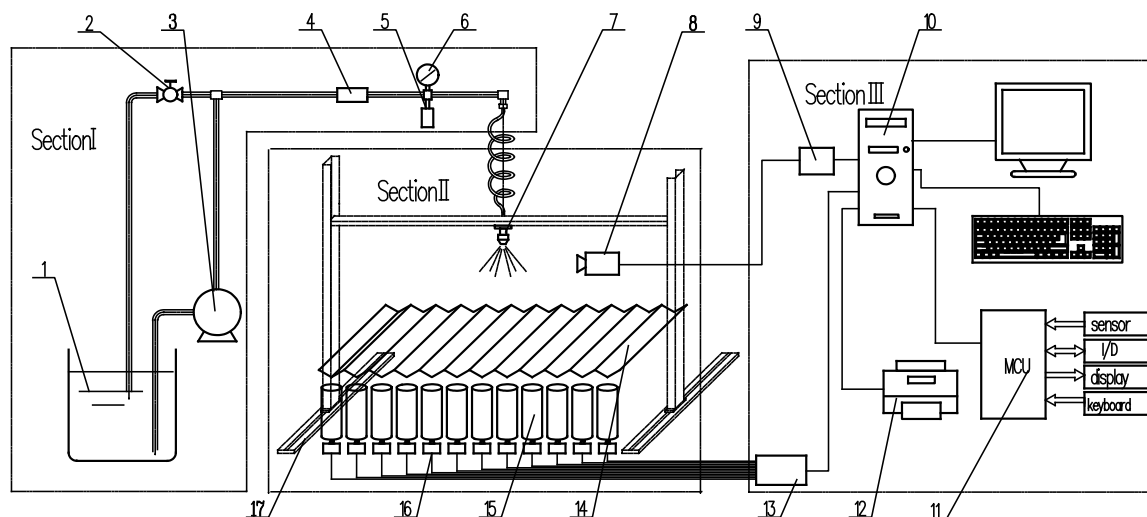
1. Tank; 2. Electric control valve; 3. Pump; 4. Flow sensor; 5. Pressure sensor; 6. Manometer; 7.Nozzle; 8. Camera; 9. Image capture card; 10. Host PC; 11. MCU; 12. Printer; 13. Data acquisition card; 14. Groove; 15. Cup; 16. R; 17. Nozzle drive rack.
